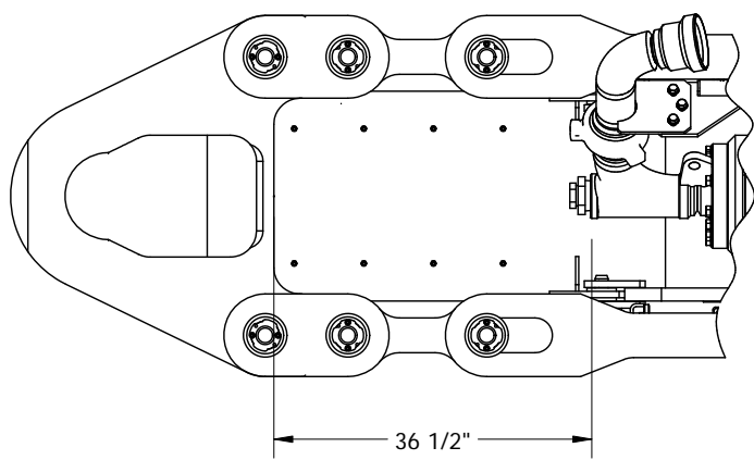
Optional Extension Links for Wireline Sheave
